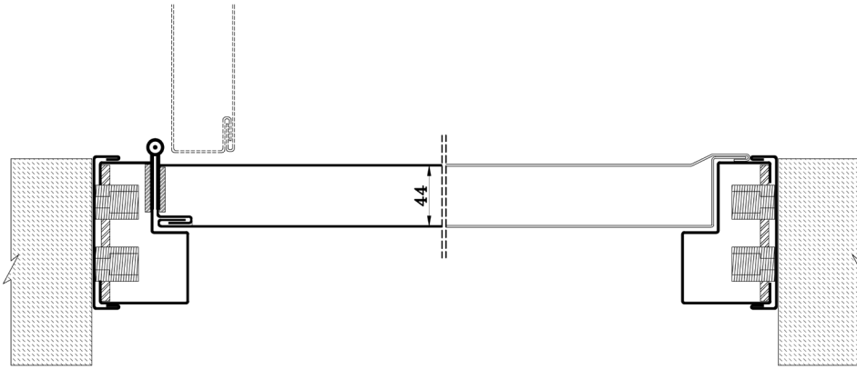
Single Door-set
