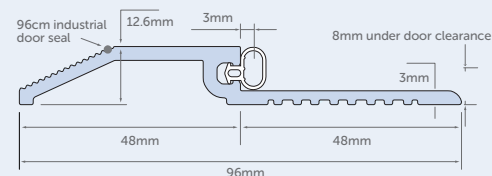
Fig. 3 Industrial door threshold - 96mm
