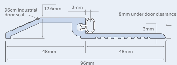
Fig. 3 Industrial door threshold - 96mm
