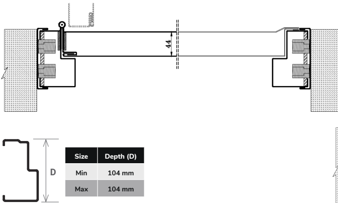
Fig. 2 3 sided single rebate frame assembly
