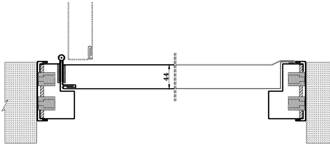
Fig.1 Single door with single rebate frame assembly
